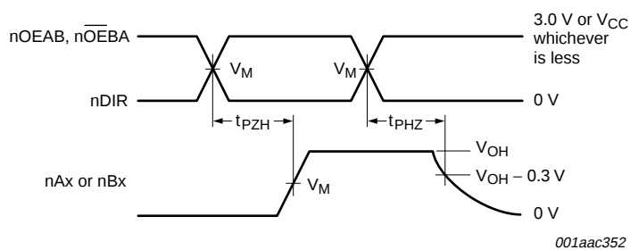
Fig 9. 3-state output enable time to HIGH-level and output disable time from HIGH-level
